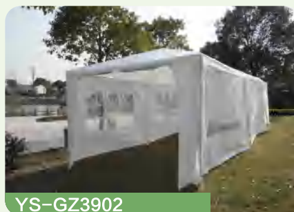
YS-GZ3902 3x9m PE gazebo with 8pcs walls Steel tube: dia31.5/24/18mm, PE connector. Fabric: 90-100g/m2 PE
